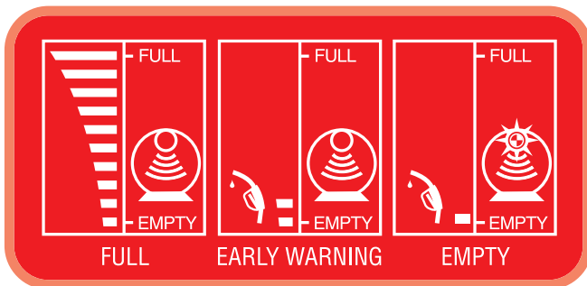
DIAGRAM 3 - Continuous display on small LCD Panel of Receiver 10 bar graph level display
